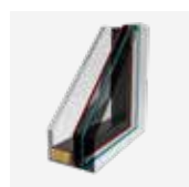
VERGLASUNG P20 U_g = 1,0 \text{ W/m}^2\text{K}
